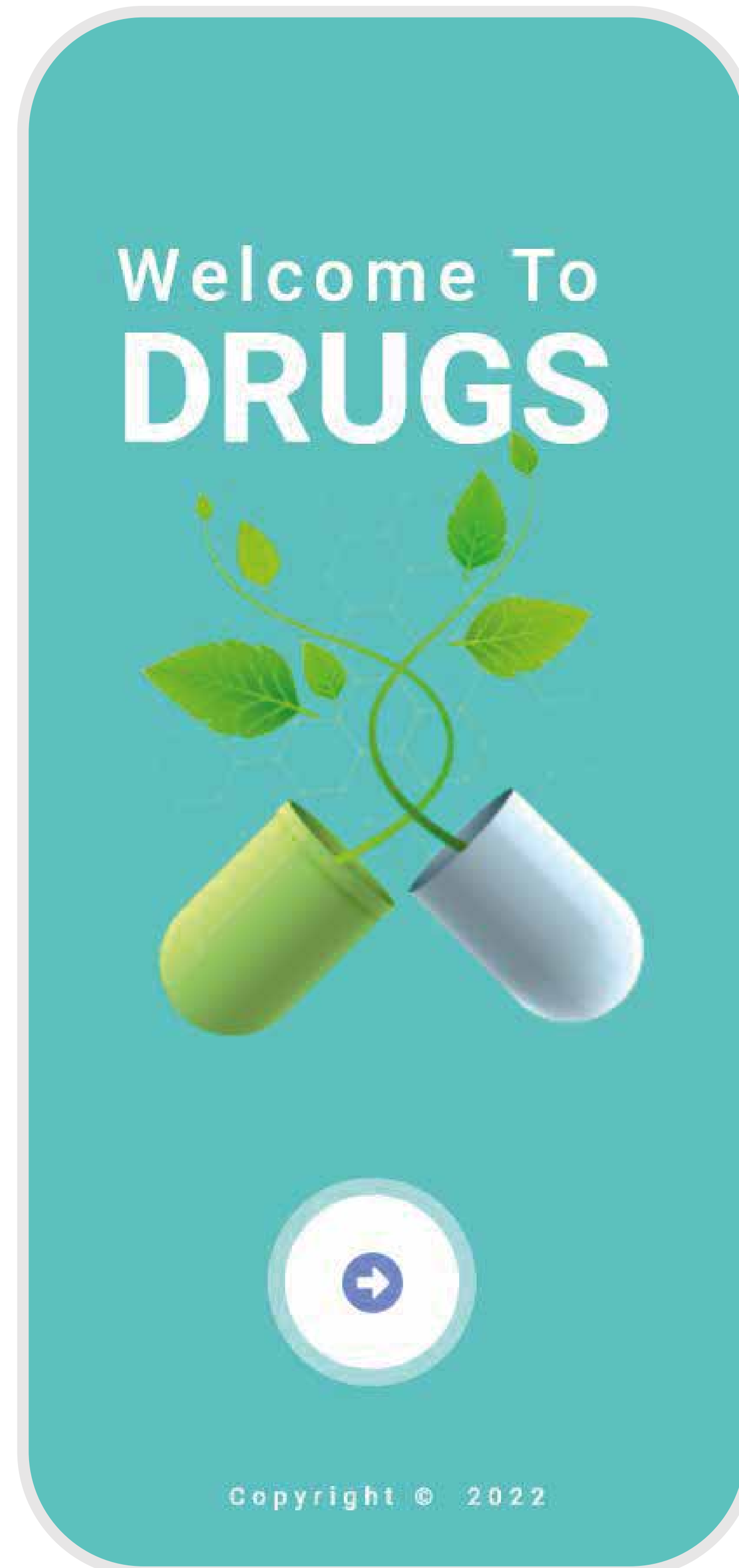
MEDICINE APP
