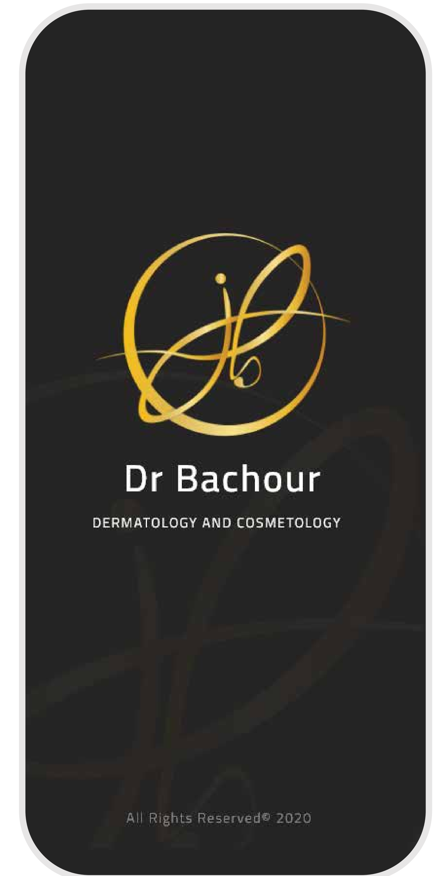
DOCTOR APP
